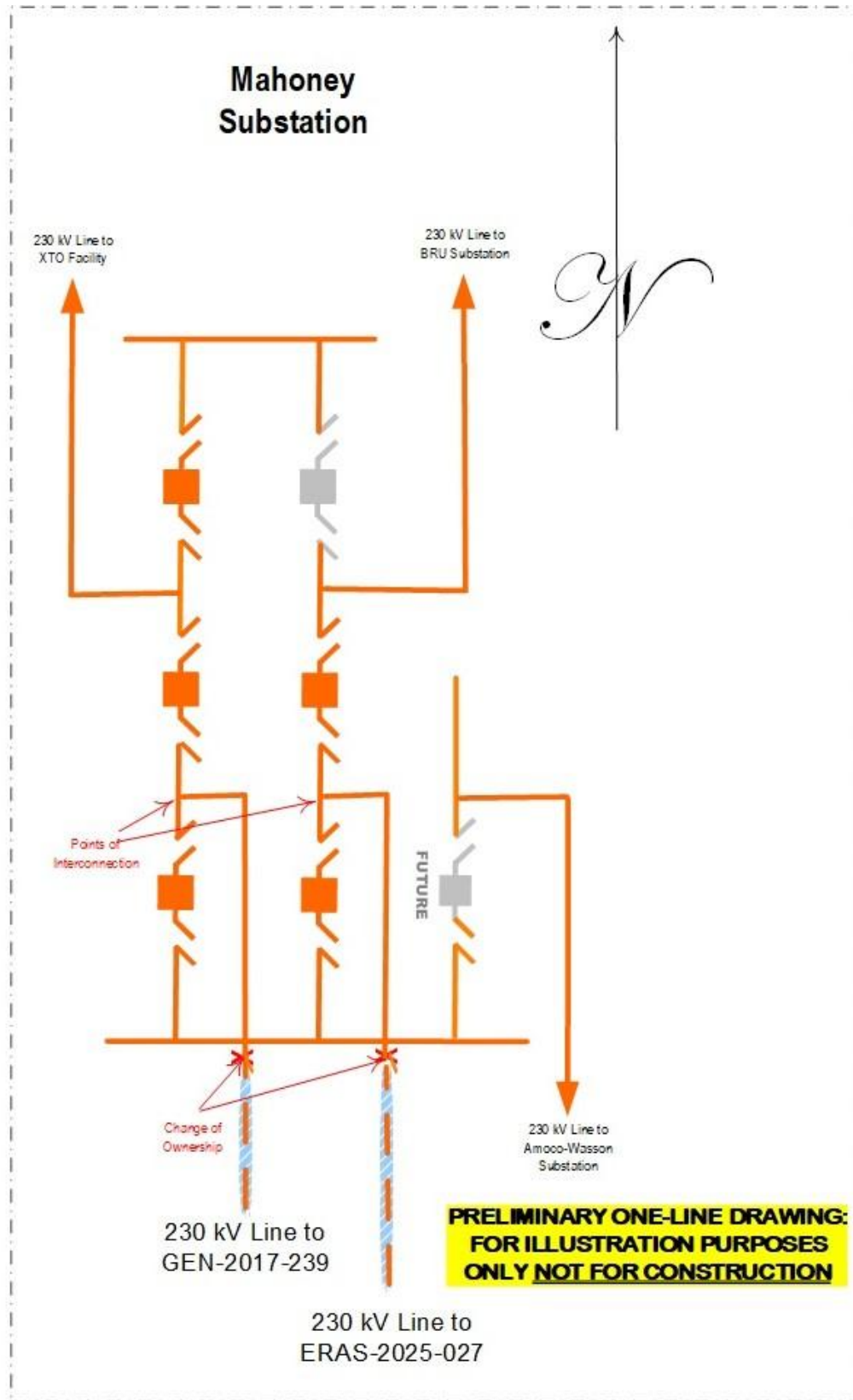
Figure A-3: Preliminary One-Line Diagram
